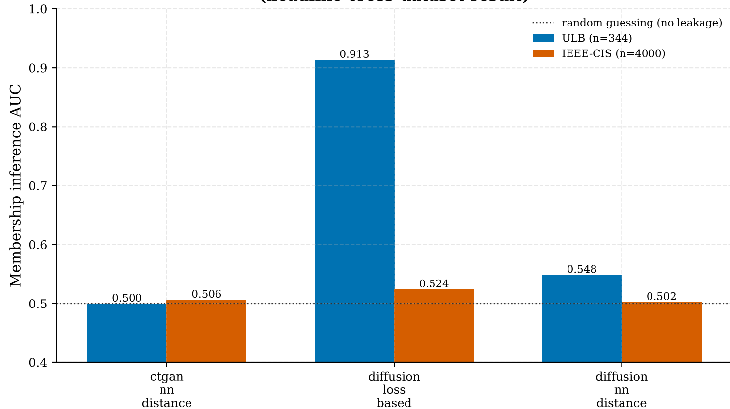
Figure 11. Membership Inference Leakage Scales Inversely with Training-Set Size (headline cross-dataset result)
